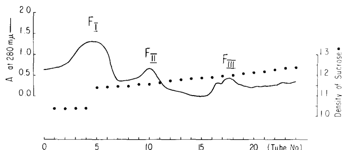
Fig. 3. A typical graph representing the distribution of subcellular fractions measured at 280 m\mu and corresponding density of sucrose in the centrifuge tube. First four points on density graph represent the loading medium of the pellet. F_I , plasma membrane; F_{II} , mitochondria and cytoplasmic membranes; F_{III} , nuclear fraction.
